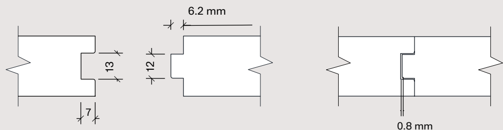
Tongue and groove detail of SuperPan® Tech for thicknesses between 25 and 40mm.
