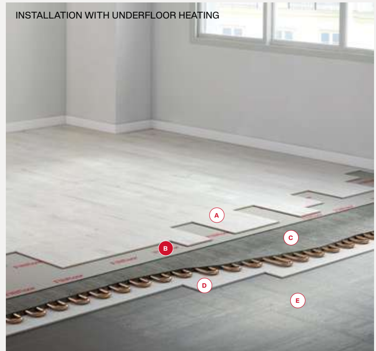
A FINFLOOR B FINFLOOR SILENT ELITE UNDERLAY C UNDERFLOOR HEATING D INSULATION E SUB-FLOOR
