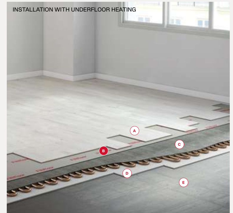
A FINFLOOR B FINFLOOR SILENT ELITE UNDERLAY C UNDERFLOOR HEATING D INSULATION E SUB-FLOOR
